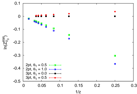
Figure 4: Tree-level continuum results for the renormalization constant of the temporal component of the vector current, \ln Z_{V_0} , in the static approximation. We compare its definition via two-point correlation functions only (2pt) with our standard definition to fix this HQET parameter, which uses three-point functions (3pt).
