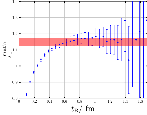
Figure 5: The ratio f_0^{\text{ratio}} (blue points) and the fit result \varphi_\mu^{(1,1)} (red band) for lattice N6, \mu = 0 and fixed t_K = 20 .
