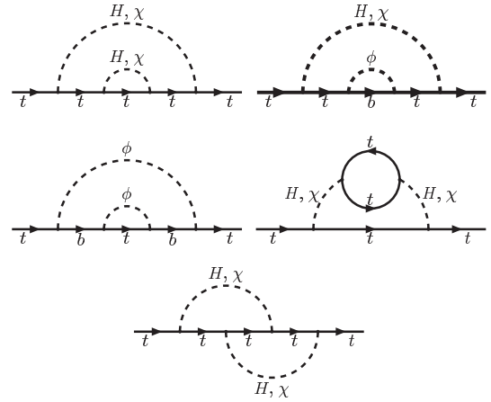
Figure 2: Two-loop on-shell diagrams which contribute to the translation of the \overline{\text{MS}} mass to the pole mass.
