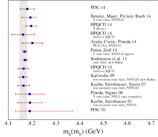
Figure 10: Comparison of m_b(m_b) with several other determinations.
