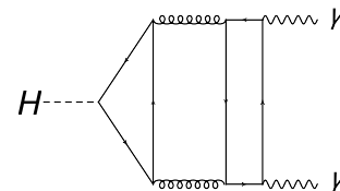
Figure 13: Example three-loop singlet diagram. Solid lines denote top quarks, wavy lines are photons, twisted lines represent gluons and the dashed line is the Higgs boson.
