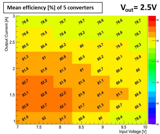
Figure 9: Mean efficiency measured on 5 converter prototypes with 2.5 V output voltage in percent as a function of input voltage and output current.
